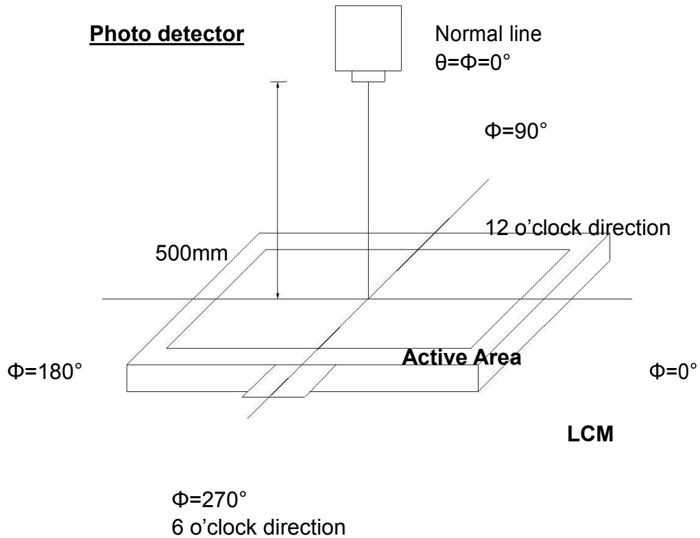
Fig. 4-2 Optical measurement system setup
